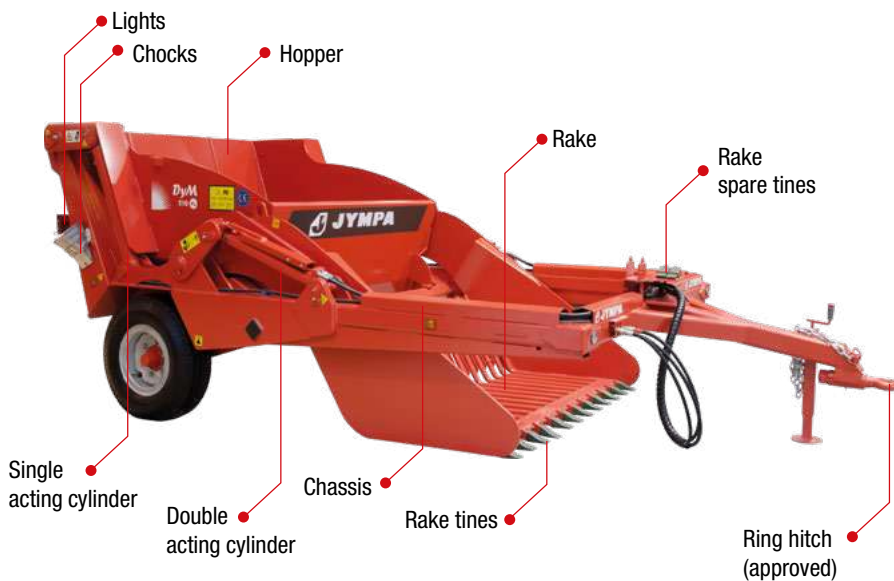
Model DYM-210-XL
