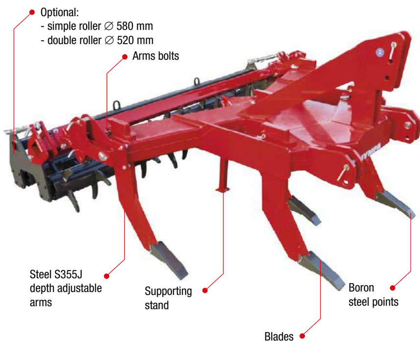
Model RIGEL-5R-2V with double roller \varnothing 520 mm
